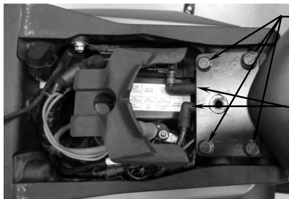
FIGURE 1 (FUEL TANK REMOVAL)
