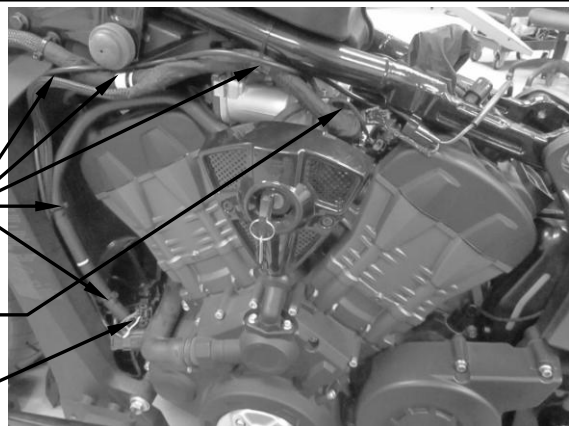
FIGURE 6 (INJECTOR & FRONT O 2 HARNES ROUTING LOCATIONS)
