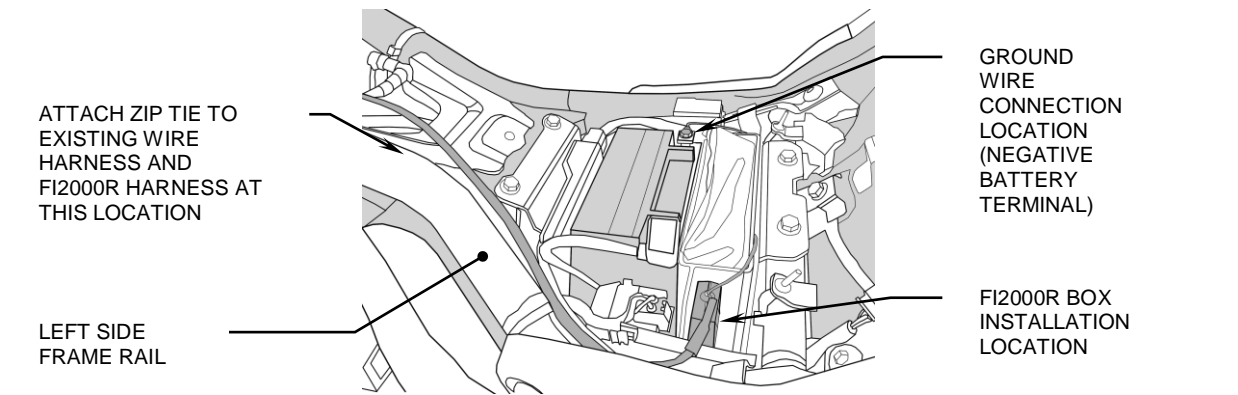
FIGURE 3: Fi2000R ECU & HARNESS INSTALLATION LOCATION AND ROUTING
