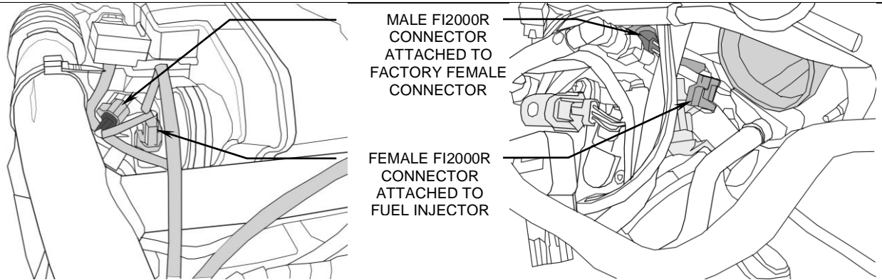
FIGURE 1: LEFT SIDE INJECTOR
